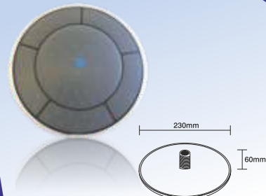
Güneş Head Shower Water Inlet 1/2
